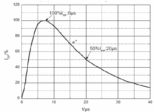
8/20 \mu\text{s} pulse waveform according to IEC 61000-4-5
