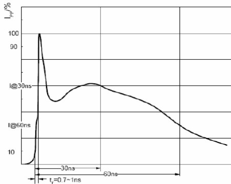
ESD pulse waveform according to IEC61000-4-2
