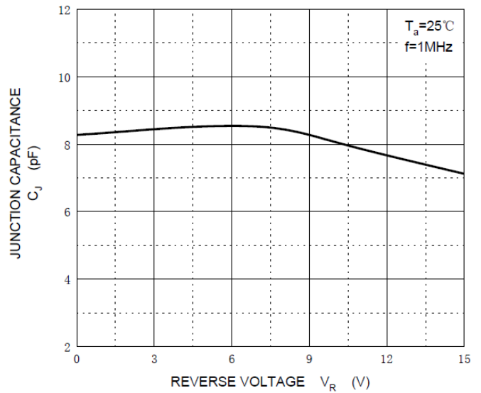
Capacitance Characteristics
