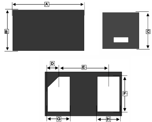
DFN1006
