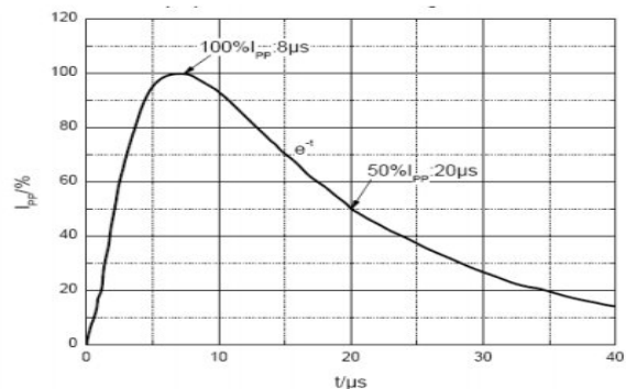
8/20µs pulse waveform according to IEC 61000-4-5
