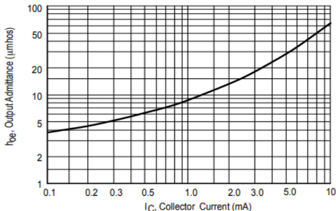
Figure 12. Output Admittance
