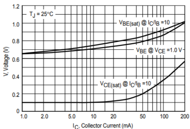
Figure 17. "ON" Voltages
