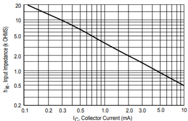
Figure 13. Input Impedance
