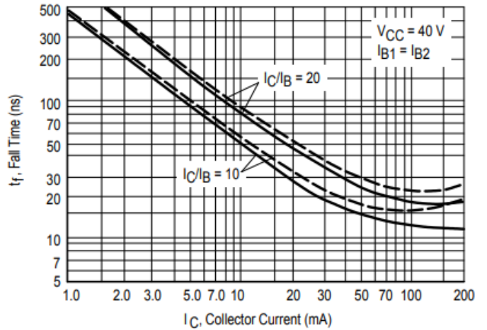
Figure 8. Fall Time
