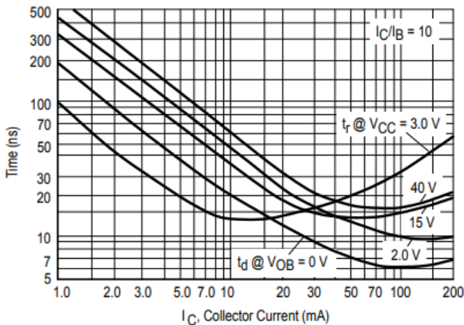
Figure 5. Turn-On Time
