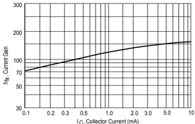
Figure 11. Current Gain
