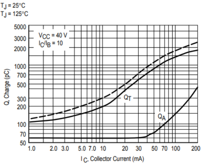
Figure 4. Charge Data
