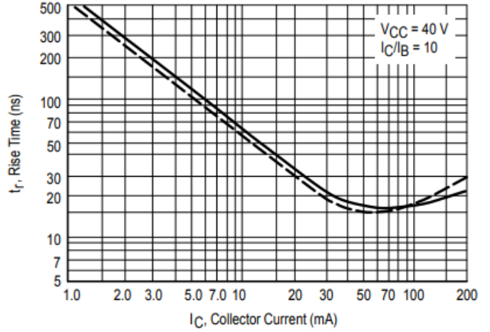
Figure 6. Rise Time
