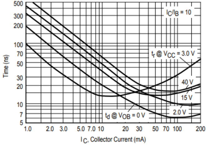
Figure 5. Turn-On Time
