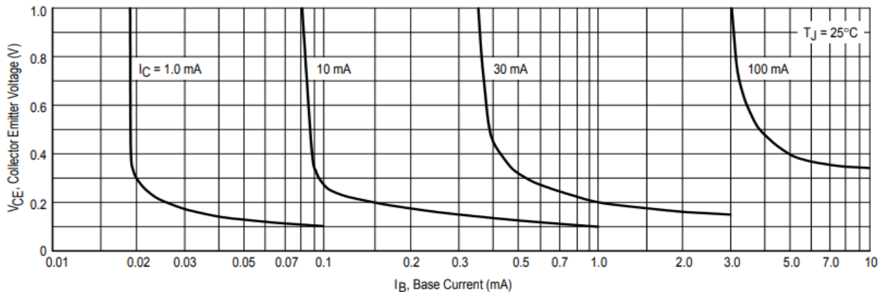
Figure 16. Collector Saturation Region
