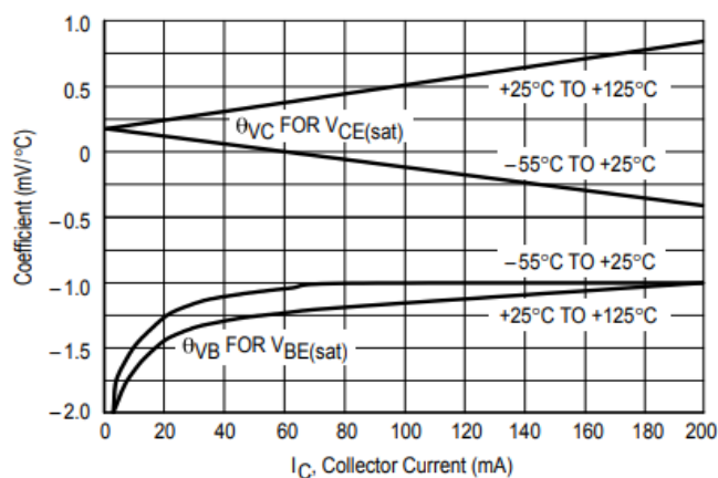
Figure 18. Temperature Coefficients
