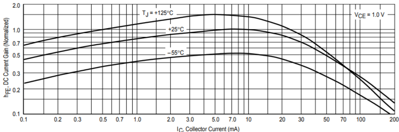
Figure 15. DC Current Gain
