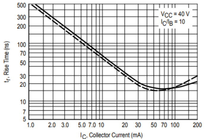
Figure 6. Rise Time
