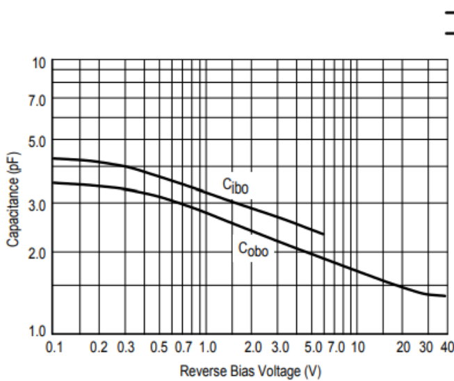
Figure 3. Capacitance
