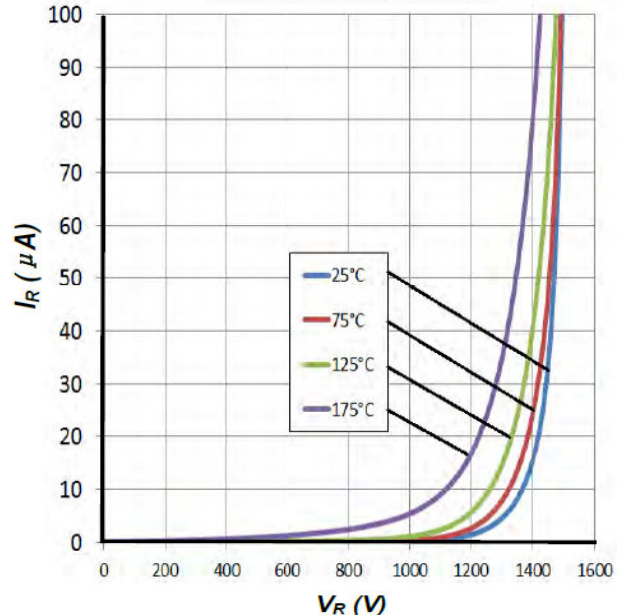
Reverse Characteristics
