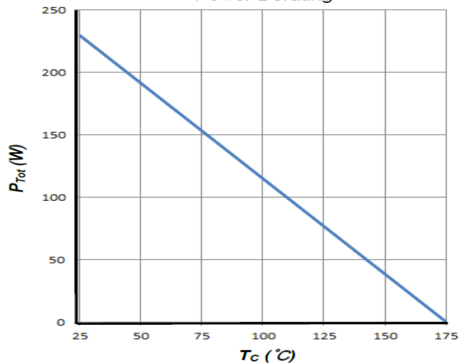
Power Derating
