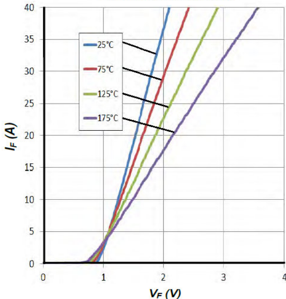
Forward Characteristics
