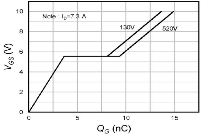
Fig.4 Gate-Charge Characteristics
