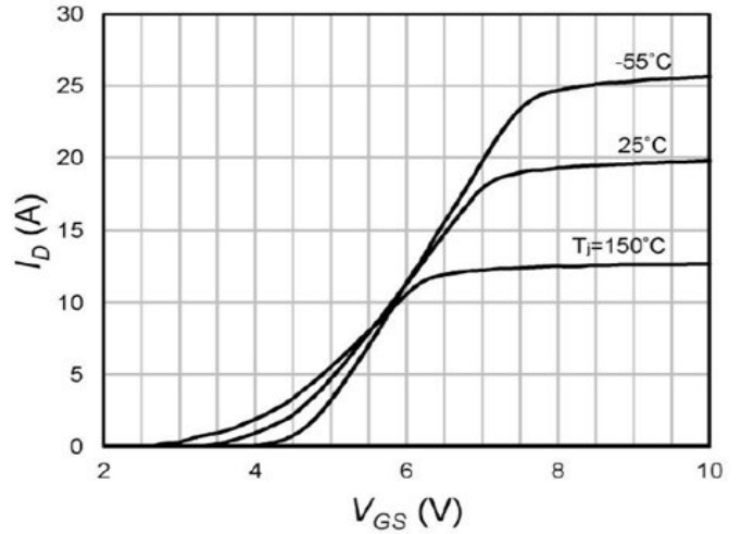
Fig.8 Transfer Characteristics
