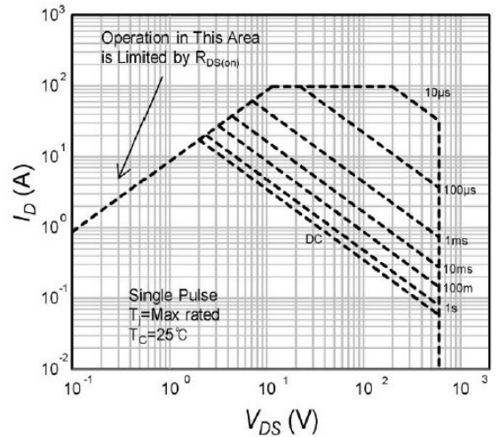
Fig.10 Safe Operating Area
