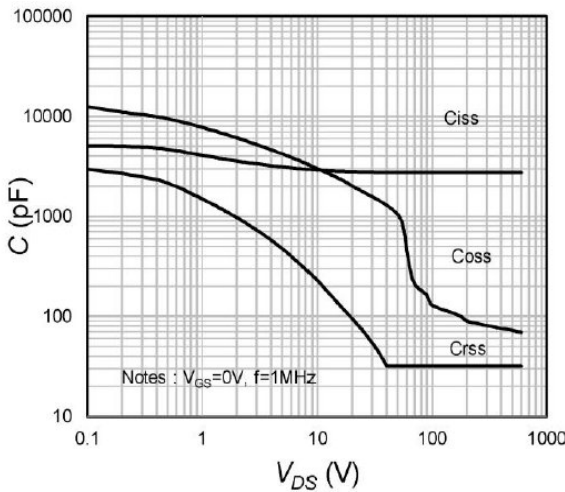
Fig.9 Capacitances
