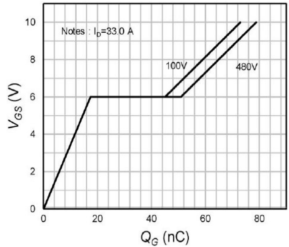
Fig.4 Gate-Charge Characteristics
