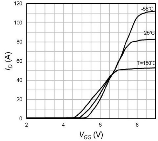
Fig.8 Transfer Characteristics
