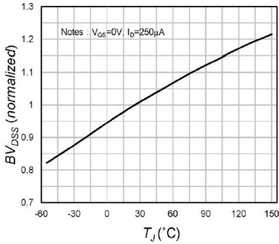
Fig.7 Drain-Source Breakdown Voltage(Normaized)
