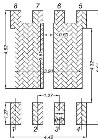
DFN5x6-8D
