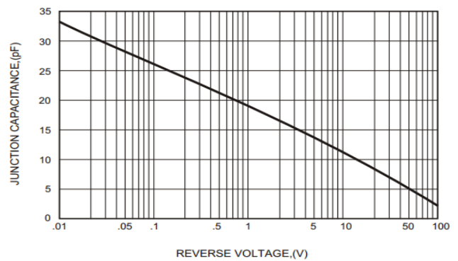
FIG.5-TYPICAL JUNCTION CAPACITANCE
